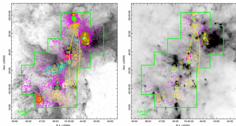
Carina Nebula
