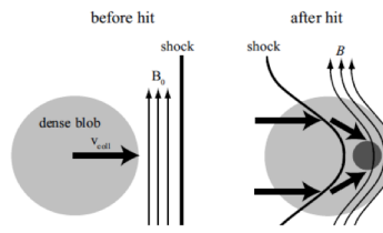
FIG. 1.— Schematics of the gas stream before (left) and after (right) the interaction between a shock and a dense blob. Because the deformed shock wave leads to a kink of stream lines across the shock, stream lines are headed toward convex point of the deformed shock wave.
